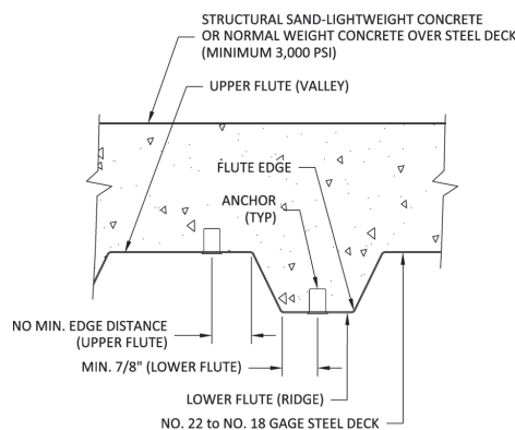
Installation Detail for Mini Dropin Installed Through Soffit of Steel Deck into Concrete
